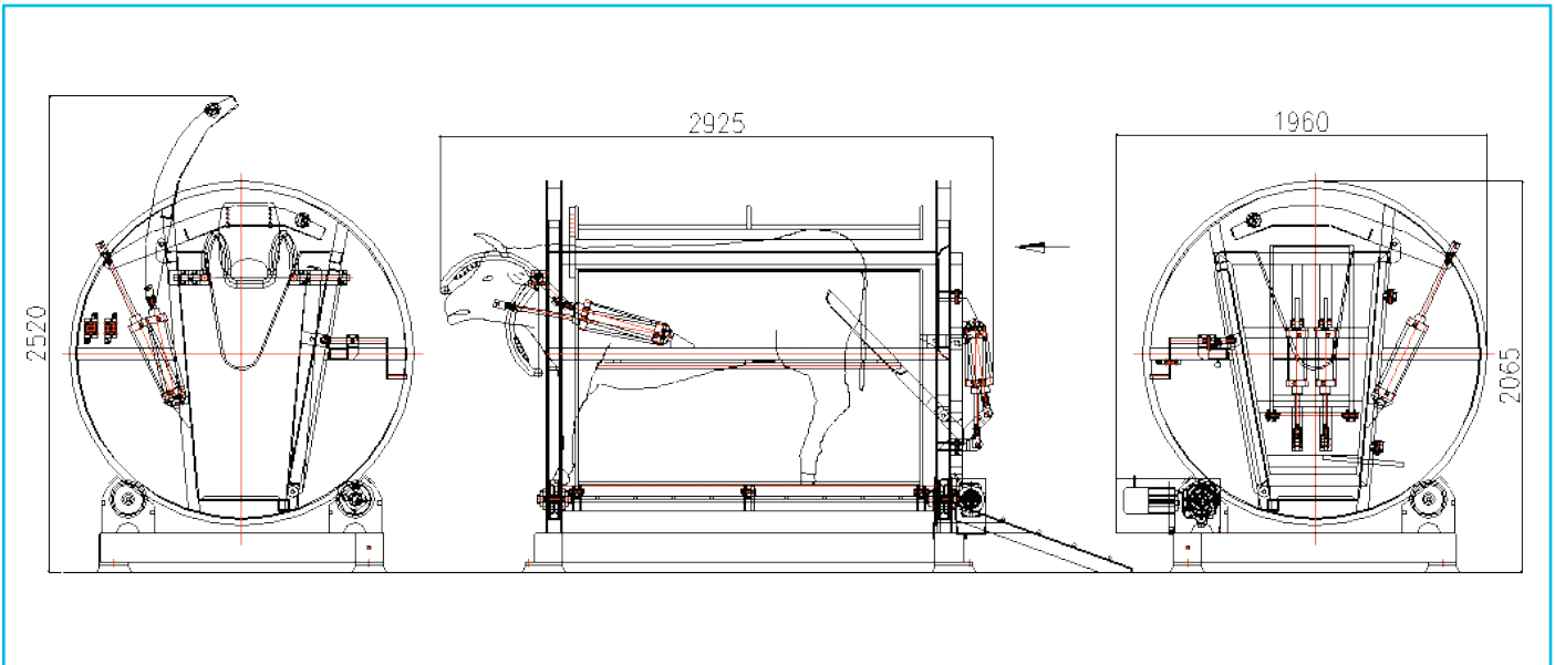
The optimal cattle dimensions for ritual stunning box type 6336220
