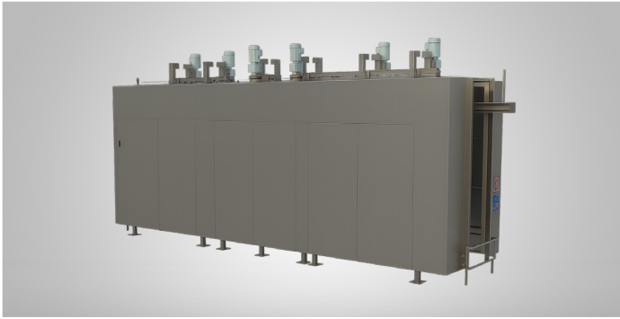
Whipping setup with 6 vertical whippers Whipping setup with 6 vertical and 6 horizontal whippers
