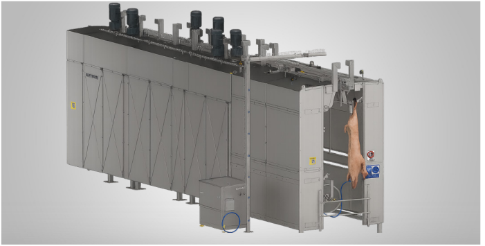
Head and hind toe brushing setup Head and hind toe brushing setup and whipping 6 vertical and 6 horizontal whippers
